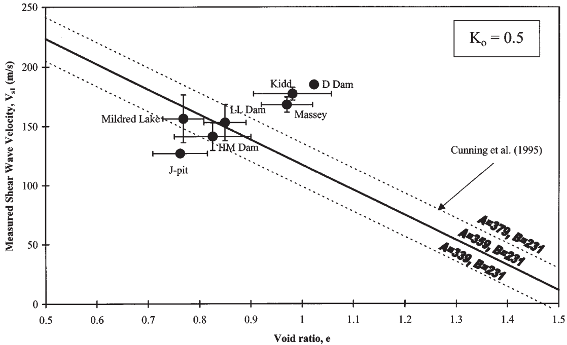
Fig. 14. Comparison of the relationship between void ratio and shear wave velocity at the CANLEX sites with the average relationship suggested by Cunning et al. (1995), adjusted to K_0 = 0.5 . Values given are averages \pm 1SD . D Dam, Duncan Dam.
