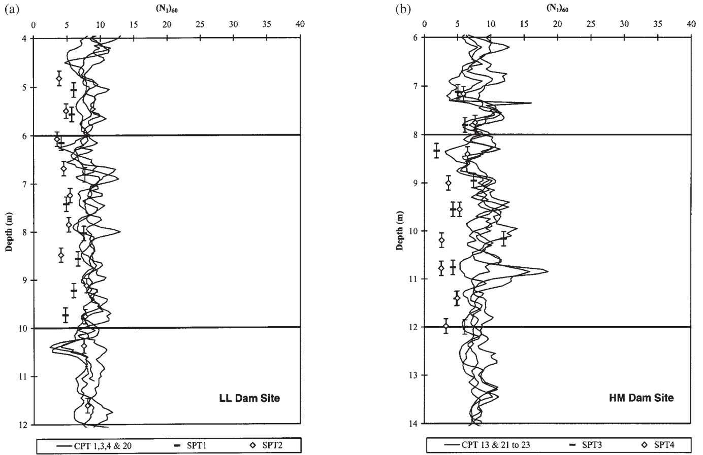
Fig. 13. Comparison of (N_1)_{60} predicted from the CPT using the equation proposed by Lunne et al. (1997) and actual SPT (N_1)_{60} results from (a) the LL Dam site, and (b) the Highmont (HM) Dam site.
