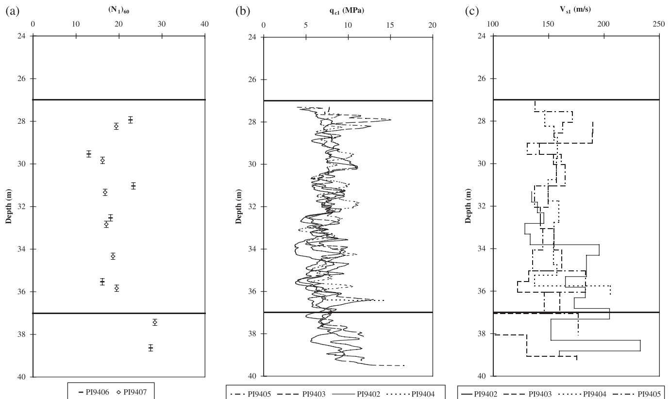
Fig. 1. Corrected (a) SPT, (b) CPT, and (c) V_{sl} profiles at the phase I (Mildred Lake) site.
