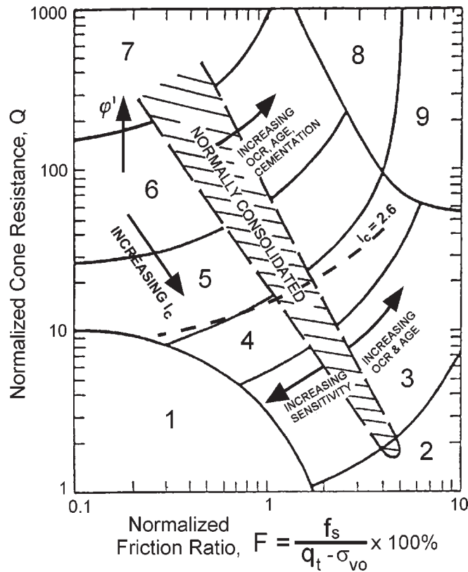
Fig. 7. Normalized CPT soil behaviour type chart after Robertson (1990): 1, sensitive, fine grained; 2, organic soils, peats (soil behaviour type index I_c > 3.6 , where I_c = [(3.47 - \log Q)^2 + (\log F + 1.22)^2]^{0.5} ); 3, clays, silty clay to clay ( 2.95 < I_c < 3.6 ); 4, silt mixtures, clayey silt to silty clay ( 2.60 < I_c < 2.95 ); 5, sand mixtures, silty sand to sandy silty ( 2.05 < I_c < 2.60 ); 6, sands, clean sand to silty sand ( 1.31 < I_c < 2.05 ); 7, gravelly sand to dense sand ( I_c < 1.31 ); 8, very stiff sand to clayey sand (heavily overconsolidated or cemented); 9, very stiff, fine grained (heavily overconsolidated or cemented). OCR, overconsolidation ratio; \phi' , friction angle.
