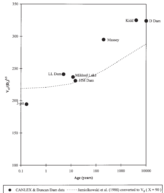
Fig. 22. Possible effects of age of deposit on measured shear wave velocity.
