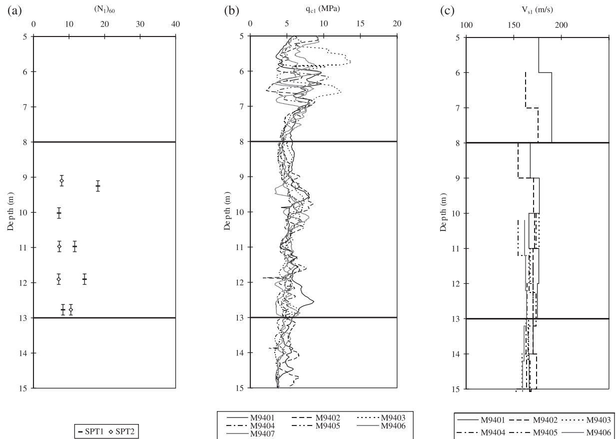
Fig. 3. Corrected (a) SPT, (b) CPT, and (c) V_{s1} profiles at the Massey site (phase II).
