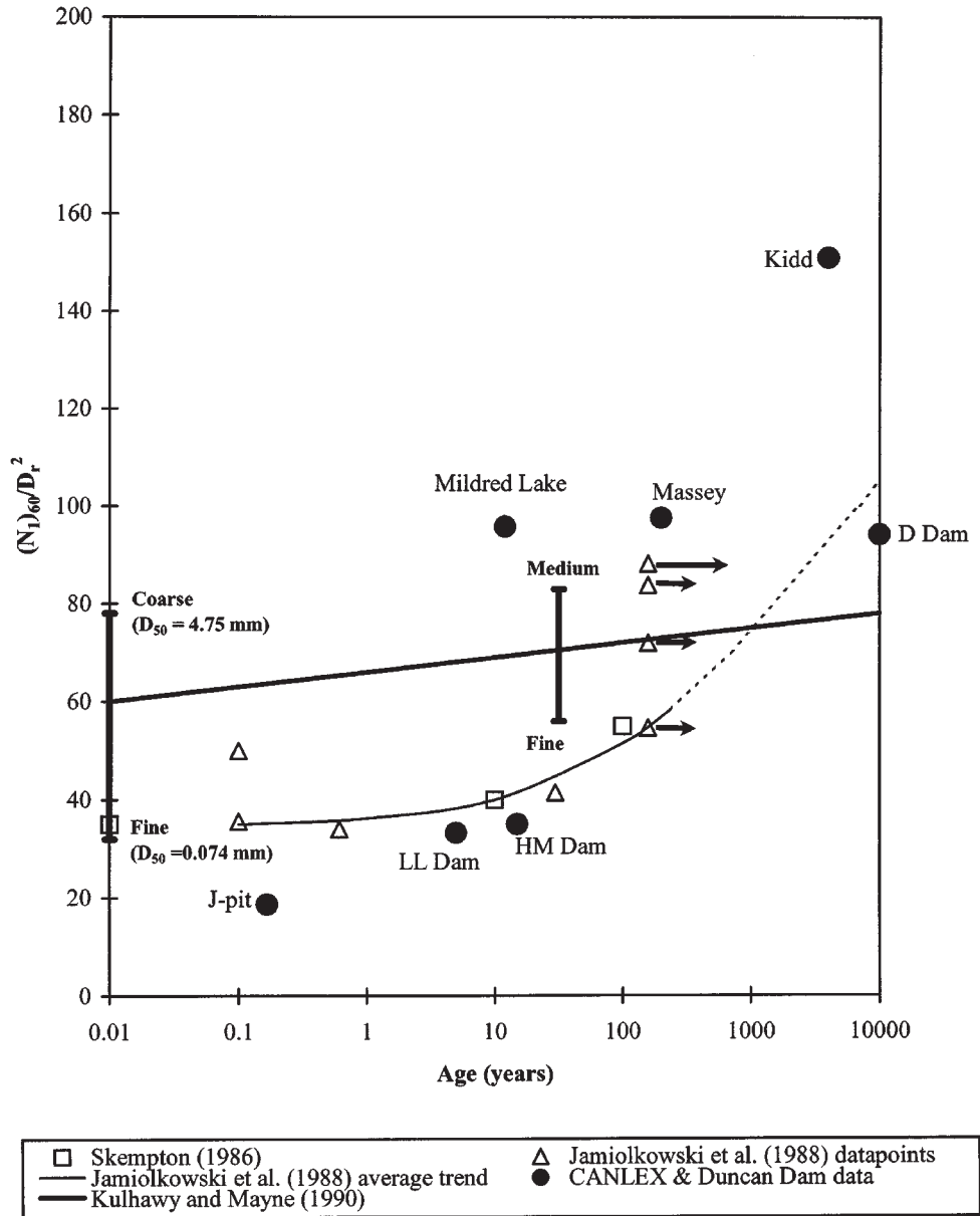
Fig. 20. Possible effects of age of deposit on SPT penetration resistance.
