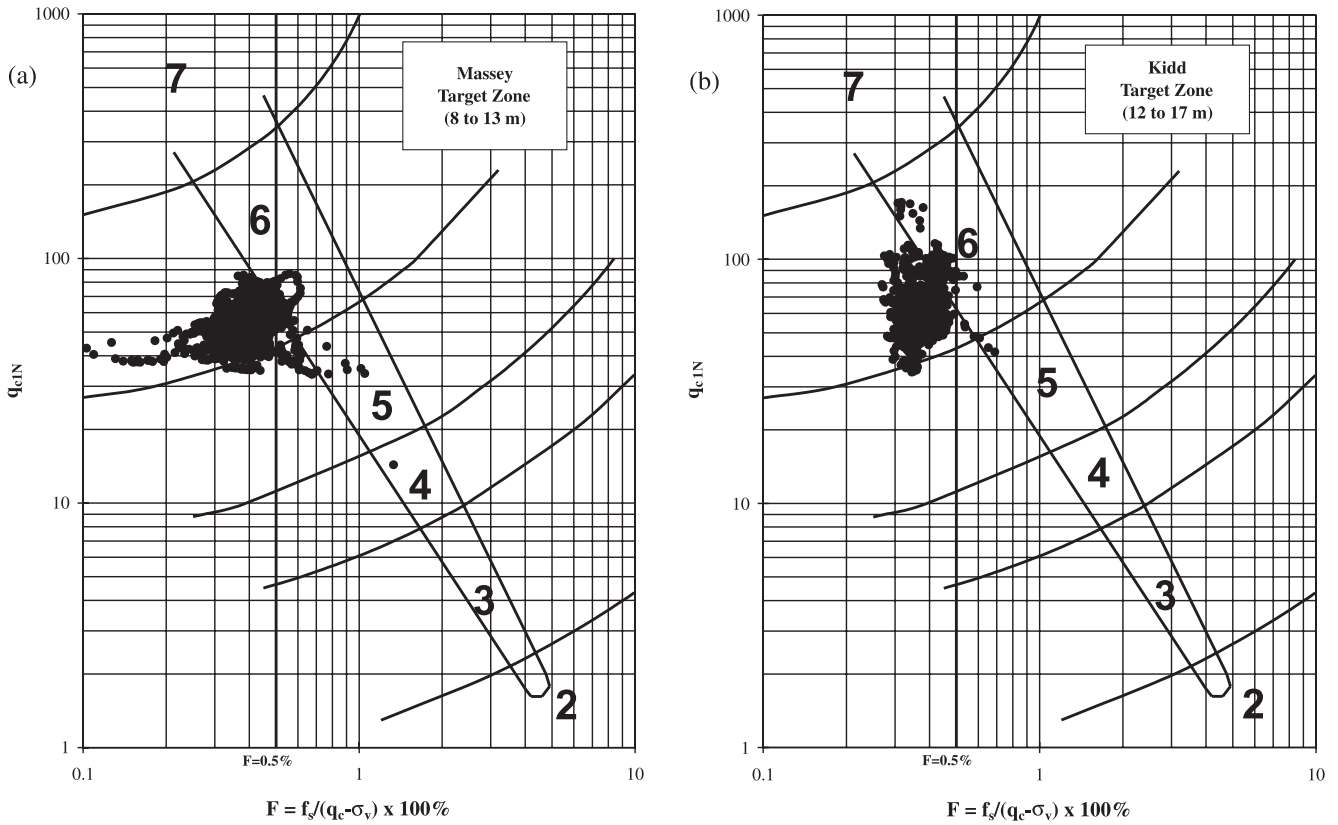
Fig. 9. CPT-based soil behaviour type classification of the phase II sites: (a) Massey, and (b) Kidd.
