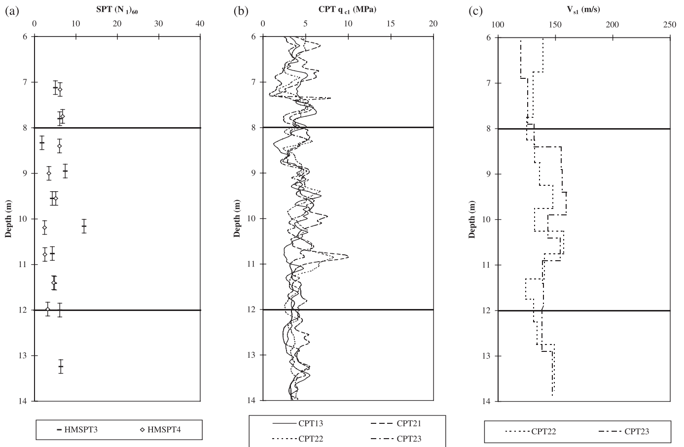
Fig. 6. Corrected (a) SPT, (b) CPT, and (c) V_{s1} profiles at the Highmont Dam site (phase IV).
