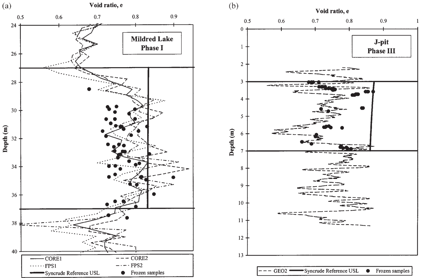
Fig. 23. Comparison of void ratio interpretation of geophysical logging results with void ratios of undisturbed ground-freezing samples from (a) the phase I site, and (b) the phase III site. FPS, fixed piston sample borehole.
