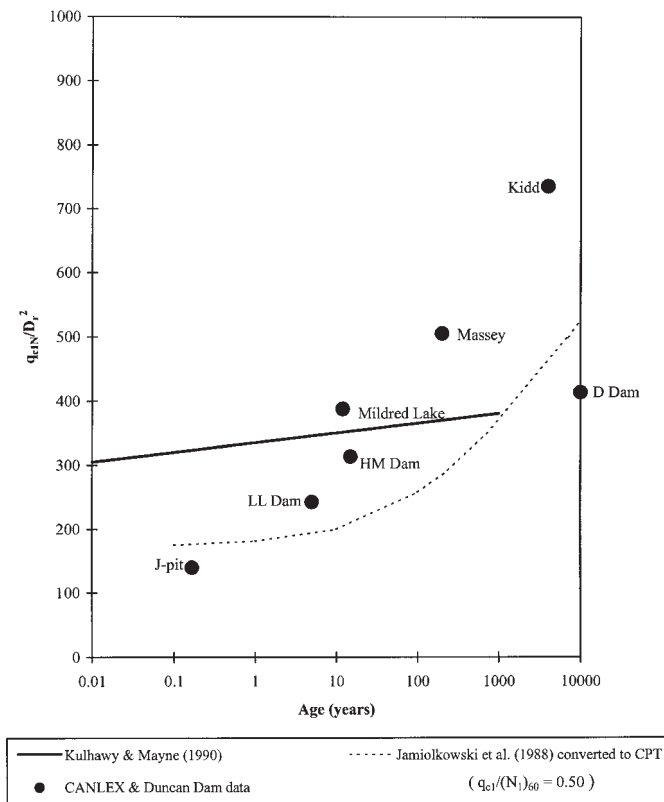
Fig. 21. Possible effects of age of deposit on CPT penetration resistance.
