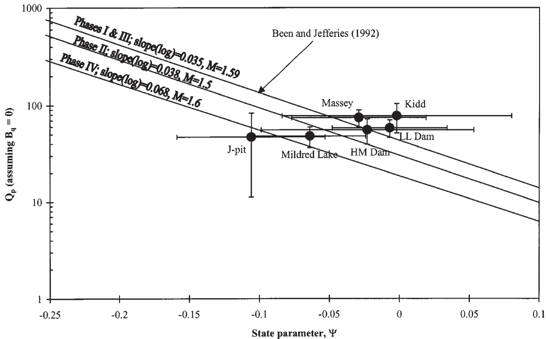
Fig. 17. Comparison of the relationships between CPT Q_p and state parameter ( \Psi ) at the CANLEX sites with the relationships based on the method by Been and Jefferies (1992), which depend on both the value of \lambda_{log} ( =2.302\lambda_{ln} , where \lambda_{ln} has been taken as the slope of the flatter portion of the reference USL) and M (which has been taken as the value of M_C ) for the particular soil.
