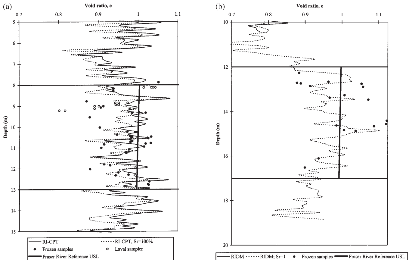
Fig. 26. Comparison of void ratio interpretation of radio-isotope CPT (RI-CPT) results (Mimura et al. 1995) with void ratios of ground-freezing samples from (a) the Massey site, and (b) the Kidd site. RIDM, radio-isotope CPT sounding.
