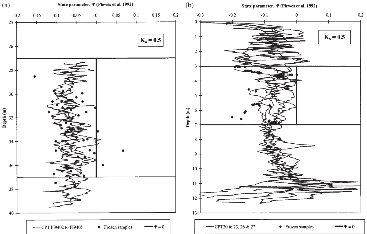
Fig. 19. Comparison of prediction of state parameter, \Psi , for Syncrude sand using the method by Plewes et al. (1992) with values of \Psi for undisturbed ground-freezing samples at (a) the phase I site, and (b) the phase III site.
