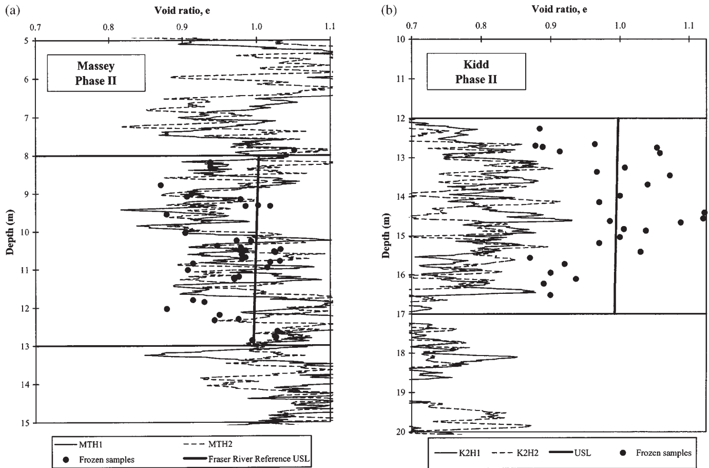
Fig. 24. Comparison of void ratio interpretation of geophysical logging results with void ratios of undisturbed ground-freezing samples from (a) the Massey site, and (b) the Kidd site. USL, ultimate state line.
