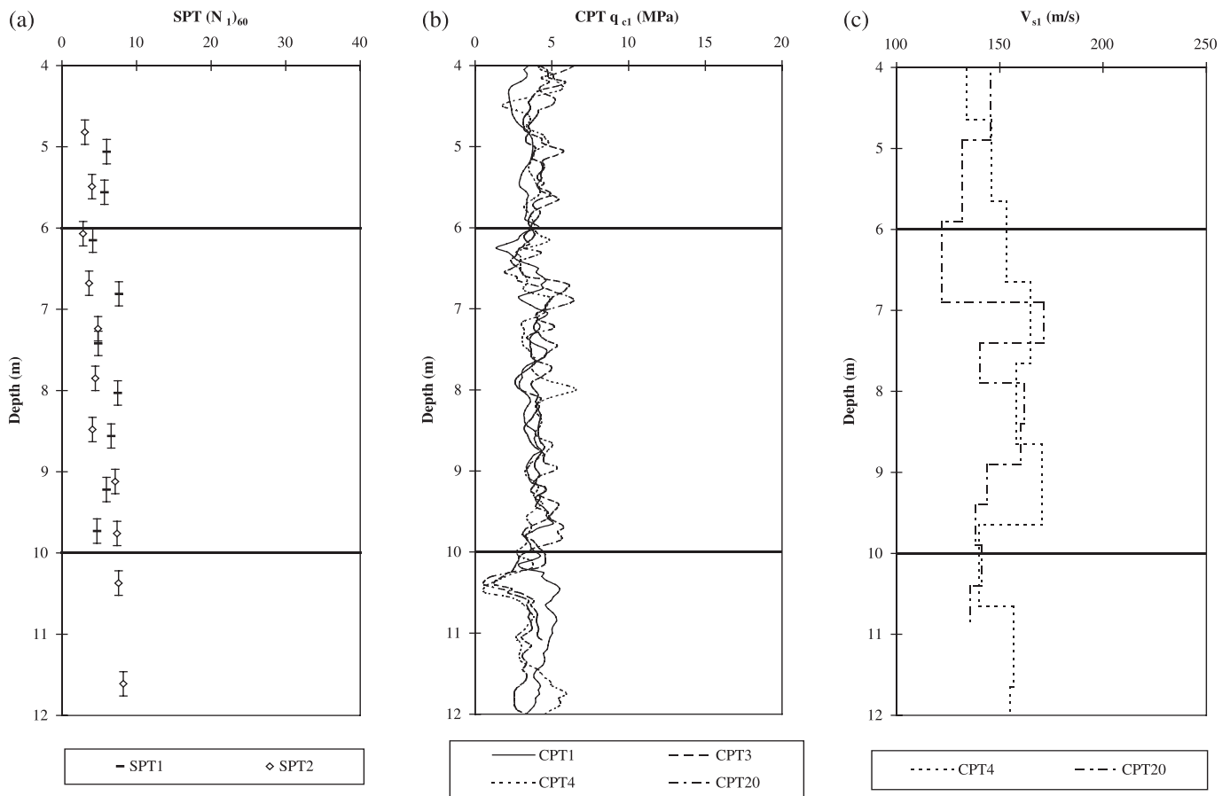
Fig. 5. Corrected (a) SPT, (b) CPT, and (c) V_{s1} profiles at the LL Dam site (phase IV).
