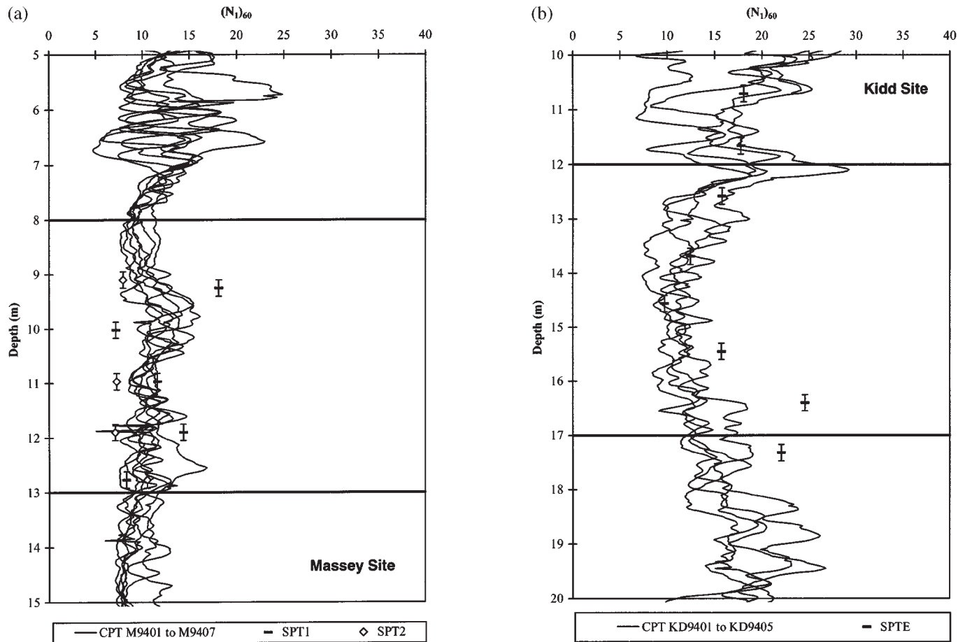
Fig. 12. Comparison of (N_1)_{60} predicted from the CPT using the equation proposed by Lunne et al. (1997) and actual SPT (N_1)_{60} results from (a) the Massey site, and (b) the Kidd site.
