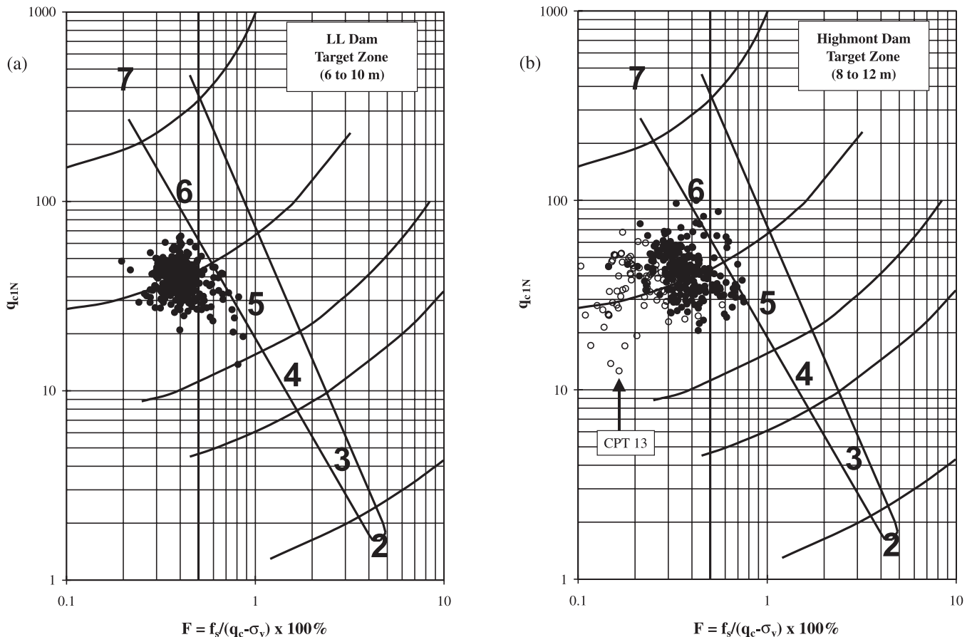
Fig. 10. CPT-based soil behaviour type classification of the phase IV sites: (a) LL Dam, and (b) Highmont Dam.
