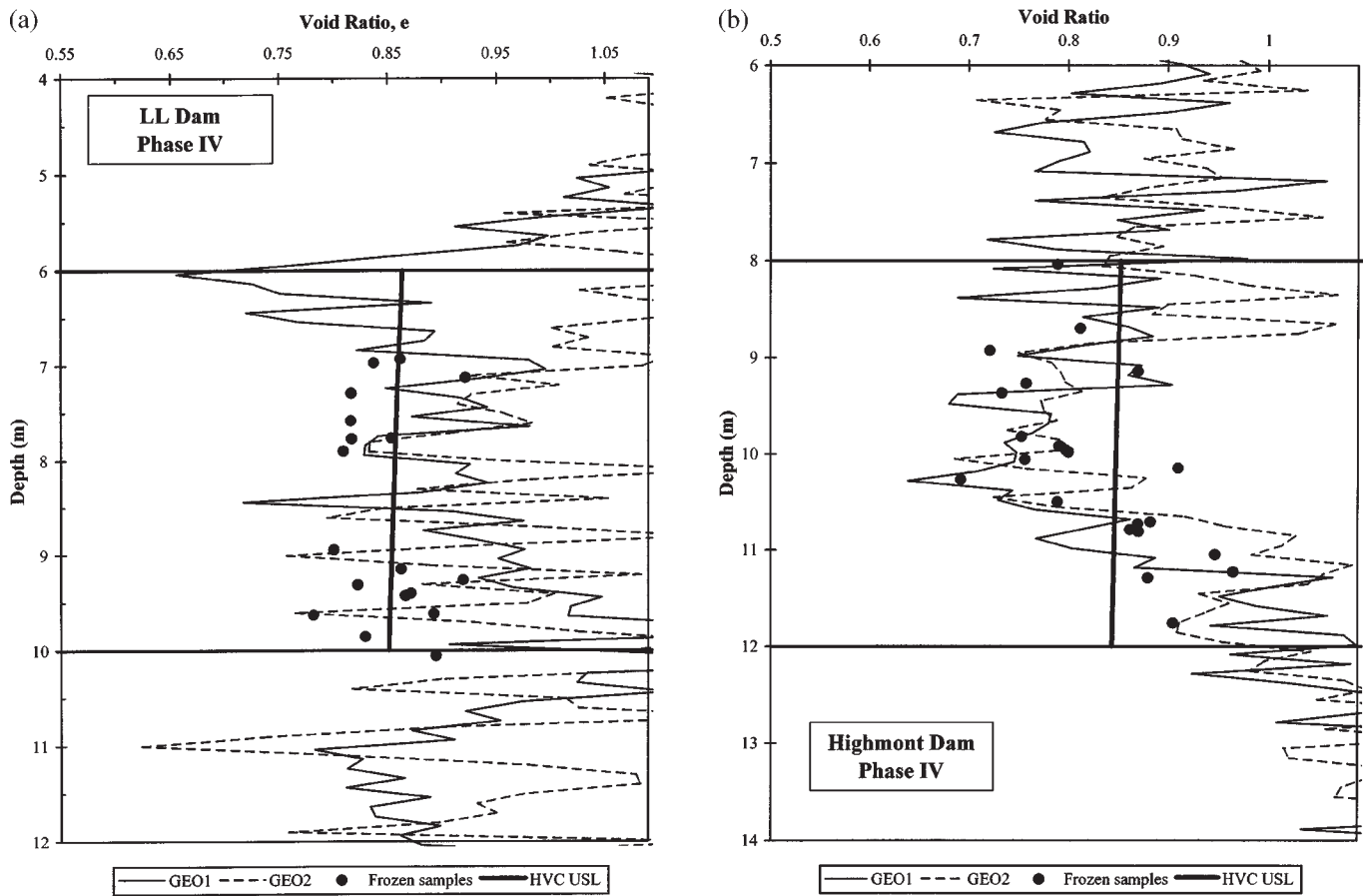
Fig. 25. Comparison of void ratio interpretation of geophysical logging results with void ratios of ground-freezing samples from (a) the LL Dam site, and (b) the Highmont Dam site. HVC, Highland Valley Copper.
