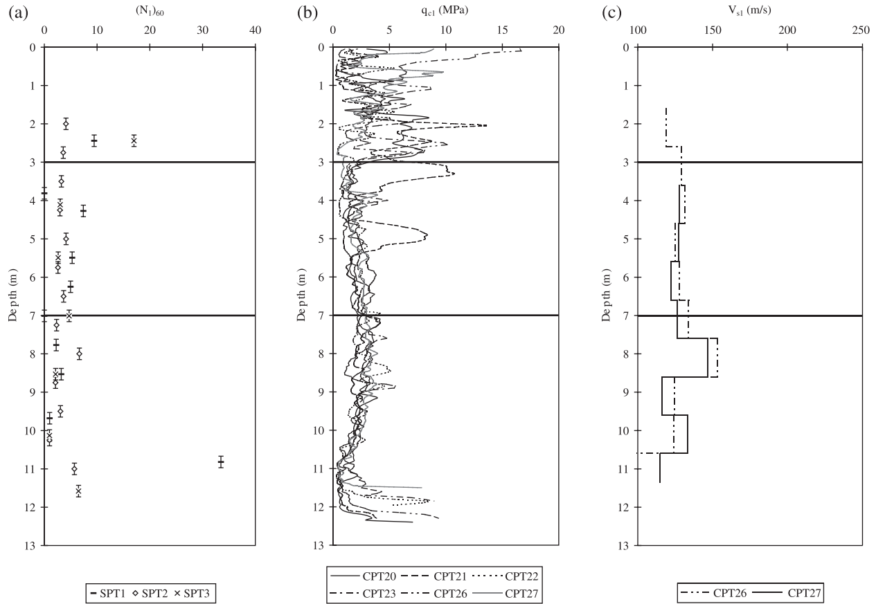
Fig. 2. Corrected (a) SPT, (b) CPT, and (c) V_{s1} profiles at the phase III (J-pit) site.
