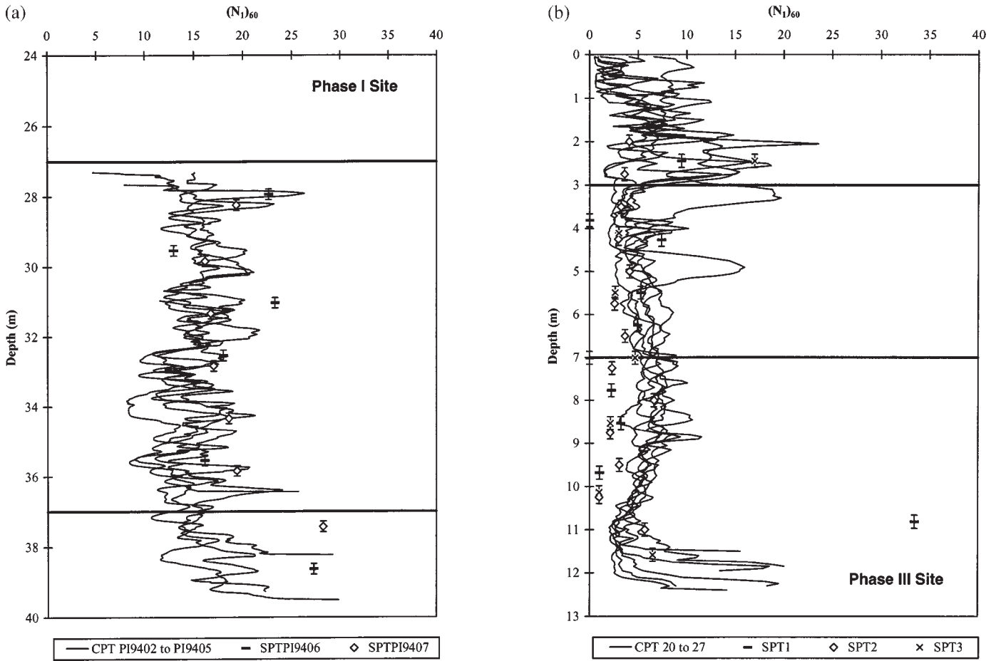
Fig. 11. Comparison of (N_1)_{60} predicted from the CPT using the equation proposed by Lunne et al. (1997) and actual SPT (N_1)_{60} results from (a) the phase I site, and (b) the phase III site.
