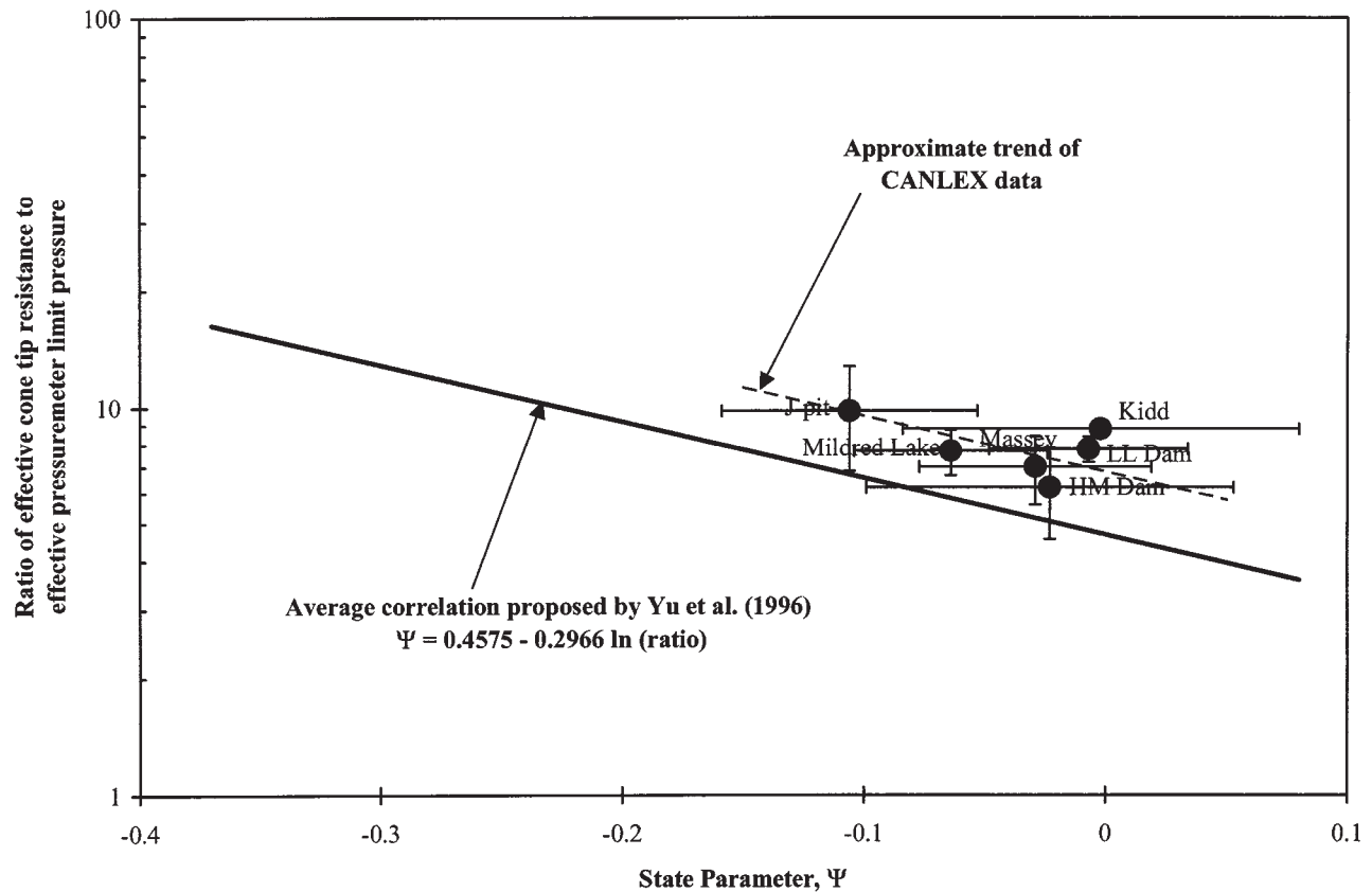
Fig. 27. Comparison of the average correlation for estimating state parameter from cone pressuremeter data, as proposed by Yu et al. (1996), with the average ( \pm 1SD ) data from the six CANLEX test sites.
