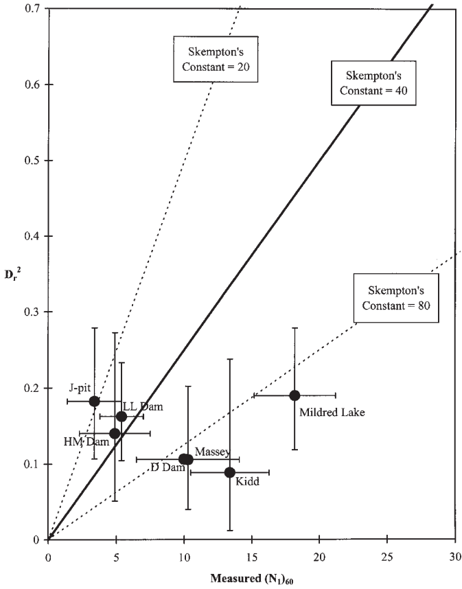
Fig. 15. Comparison of CANLEX data with relationships between SPT ( N_1 ) 60 and relative density ( D_r ) suggested by Skempton (1986). Values given are averages \pm 1SD.
