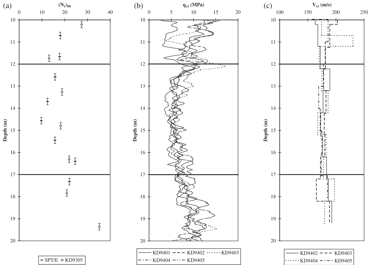
Fig. 4. Corrected (a) SPT, (b) CPT, and (c) V_{s1} profiles at the Kidd site (phase II).
