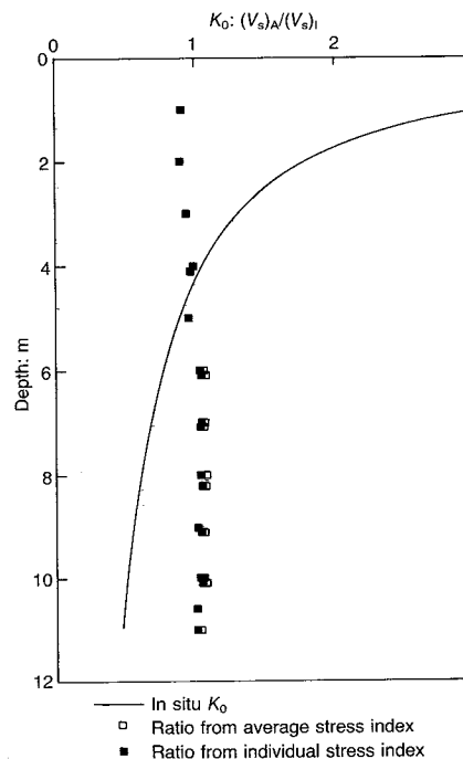
Fig. 15. Profile of K_0 and (V_s)_A/(V_s)_I at 200 St; C_A/C_I = 1
