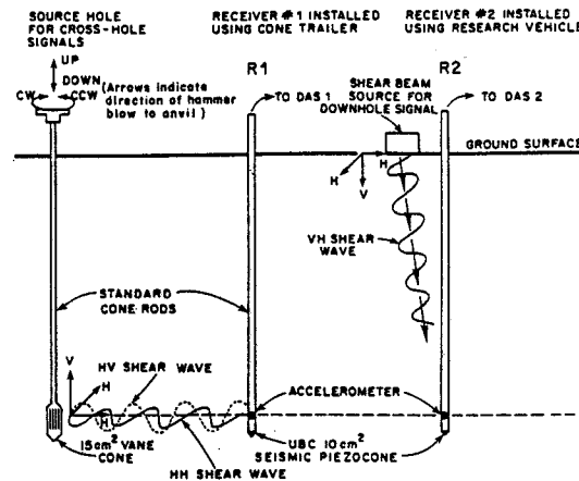
Figure 1. SCPT layout for DH and XH shear wave velocity measurements.
