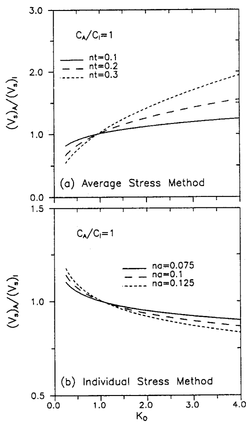
Figure 3. Theoretical dependence of (V_s)_A/(V_s)_I on K_0 .
