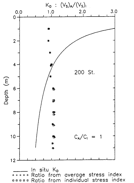
Figure 4. Profile of K_0 and (V_s)_A/(V_s)_I at 200 St.
