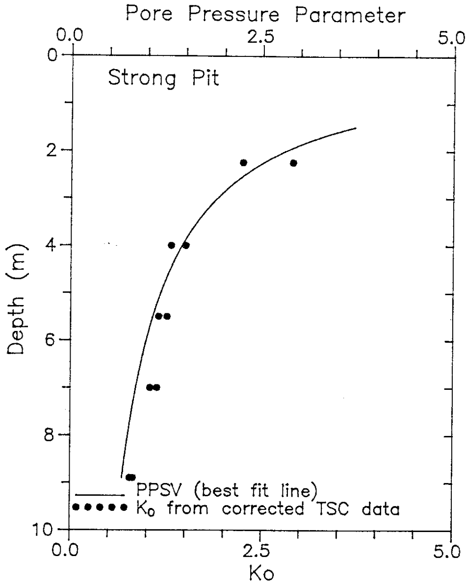
Fig. 8 Correlation between PPSV and K_o for Strong Pit.
