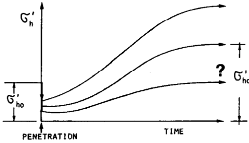
Fig.1. Schematic Diagram illustrating the variation of \sigma'_h at the Interface caused by the Pile Installation.
