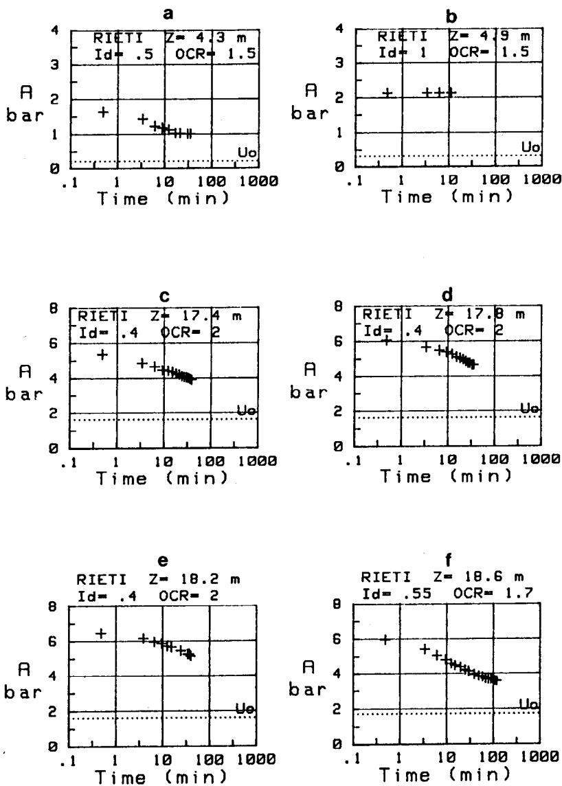
Fig.4 Reconsolidation Test Results at Rieti
